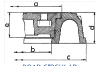
ROAD CIRCULAR MANHOLE COVER
